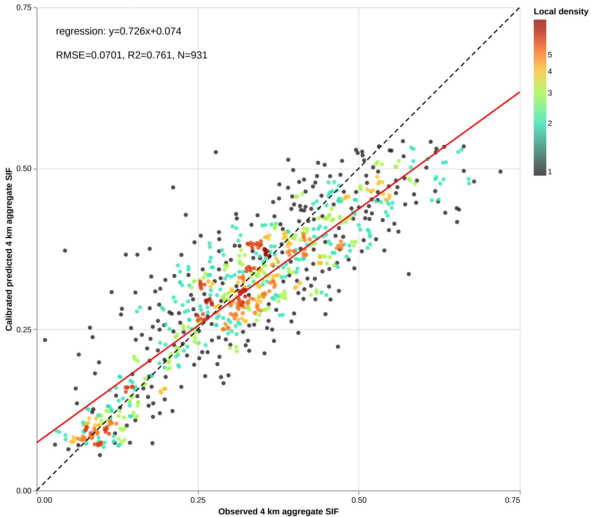
4km-Spatial-Aggregate: Observed vs. Predicted SIF, Test RMSE=0.0701, R2=0.761
